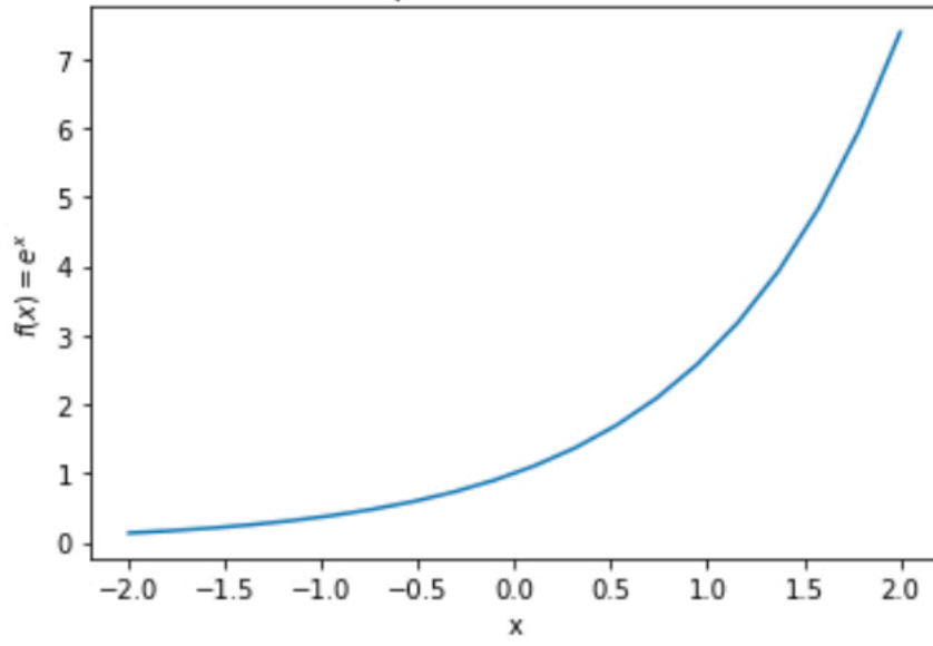
Exponential function
