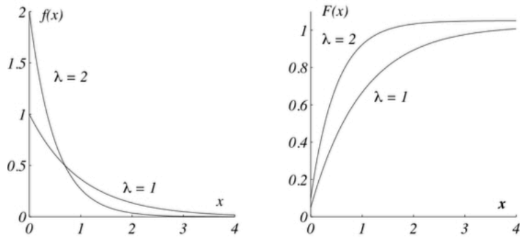
FIGURE 2 – Loi exponentielle
